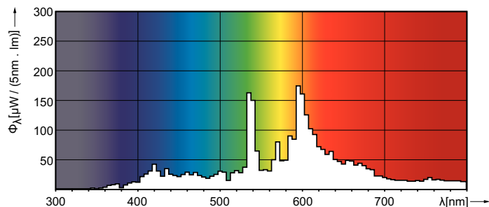
MASTERColour CDM-TD /830
