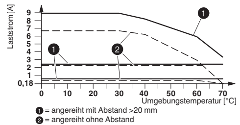
Derating-Diagramm
