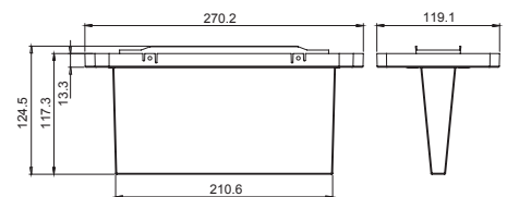
SafeLite Cone Diffuser
