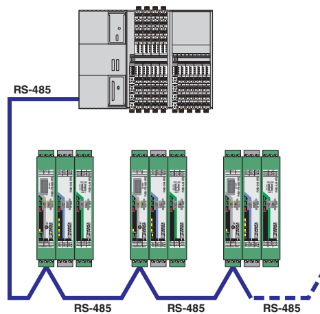
Modbus/RTU-Slave
