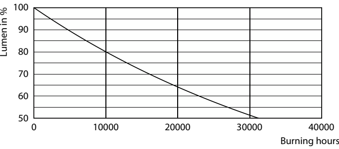
Lumen Maintenance Diagram - CorePro LEDspot 4-50W GU10 827 36D DIM
