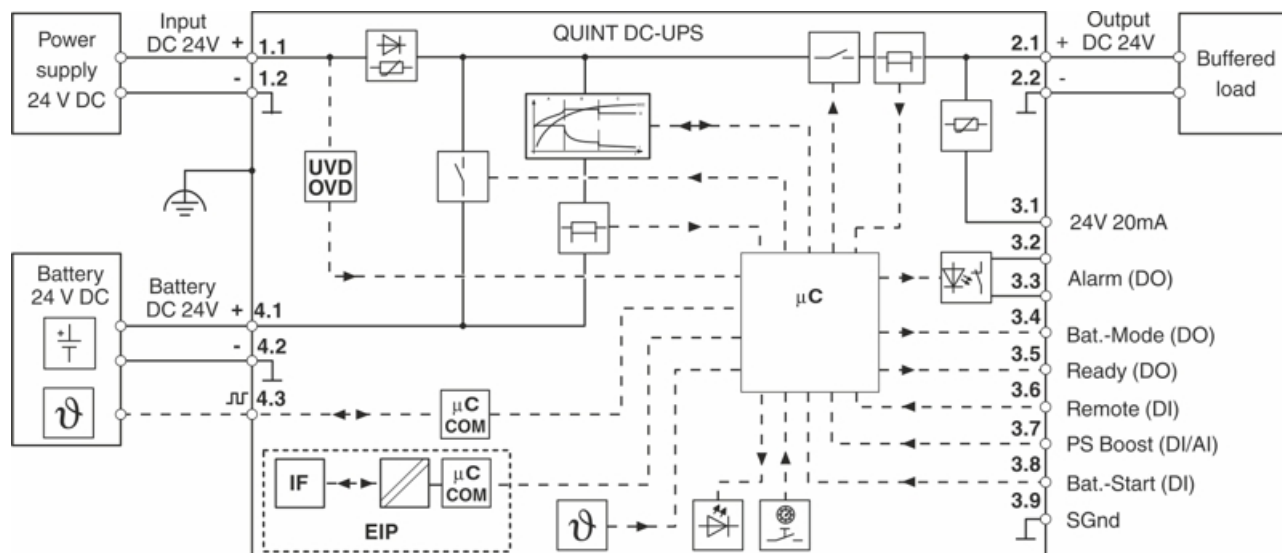
Block diagram
