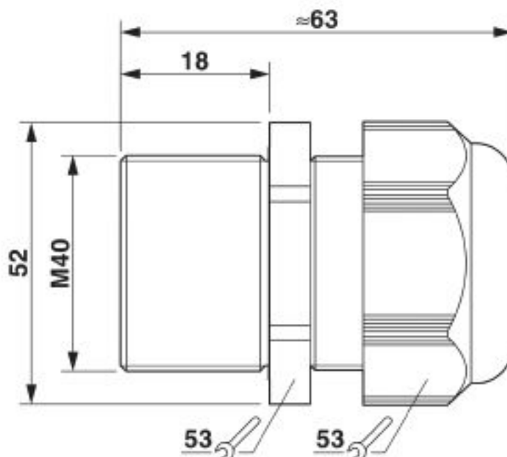
Dimensional drawing
