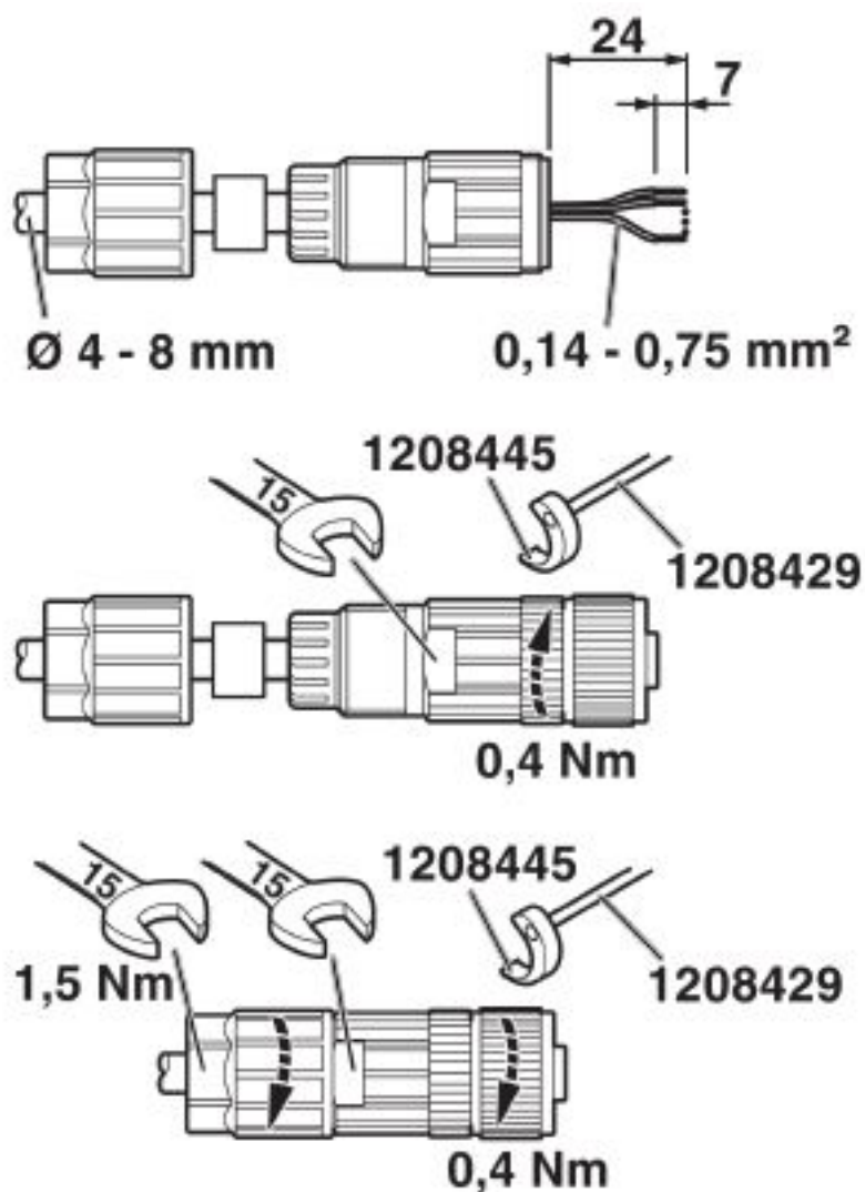
Functional drawing
