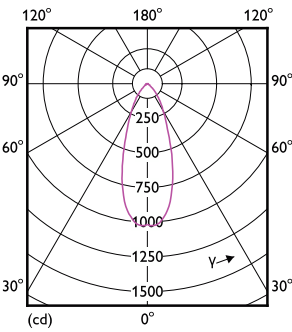
Light Distribution Diagram - CorePro LED spot ND 7-50W MR16 827 36D
