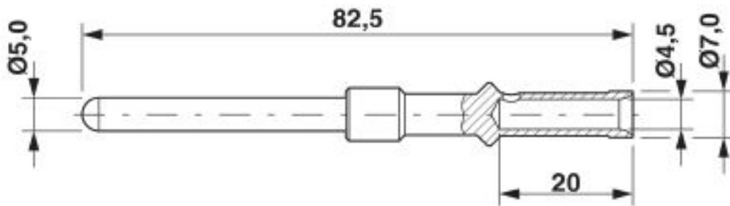
Dimensional drawing
