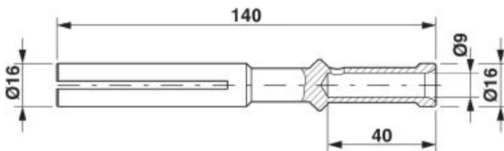
Dimensional drawing
