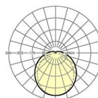
PGPC-DV/1200 LED 4100 lm 840
