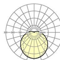
PSO/1500 LED 5800 lm 840
