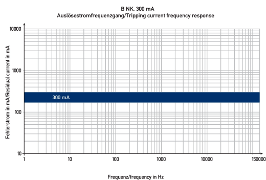
Diagramme FI-/LS-Kombinationen DRCBO 4 C16/0,30/1N-B NK
