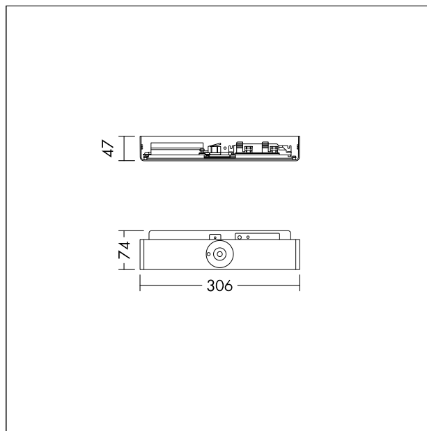
TE_ROXY_M_E3_PLUG_PLAY.wmf
