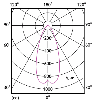
Light Distribution Diagram - MAS LED SPOT VLE D 7.5-50W MR16 930 36D
