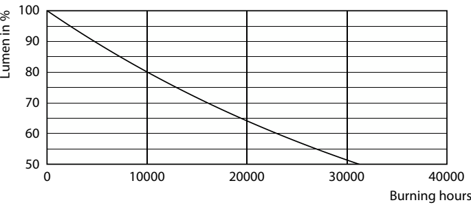
Lumen Maintenance Diagram - CorePro lustre ND 7-60W E27 827 P48 FR
