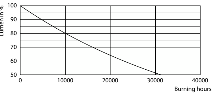
Lumen Maintenance Diagram - CorePro LEDcapsuleLV 1.7-20W G4micro 827
