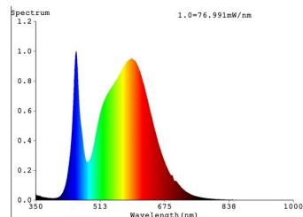
LED-Retrofit-Lampen 4000K
