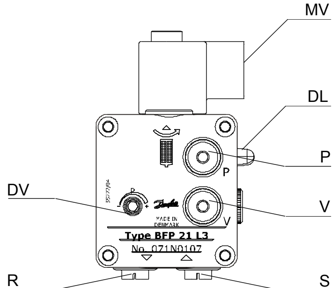
Abb. 11: Danfoss Ölpumpe BFP 21 L3 (7-15 bar)
